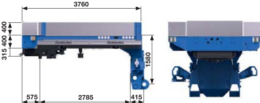
UNIVERSAL GOOSENECK
