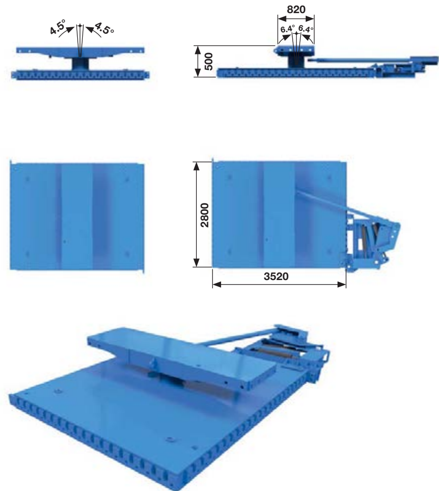
300 T/400 T TURNTABLE
