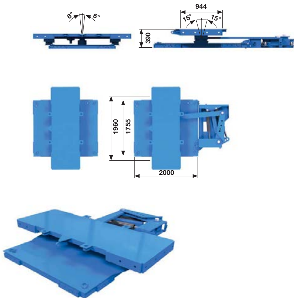
100 T/200 T TURNTABLE
