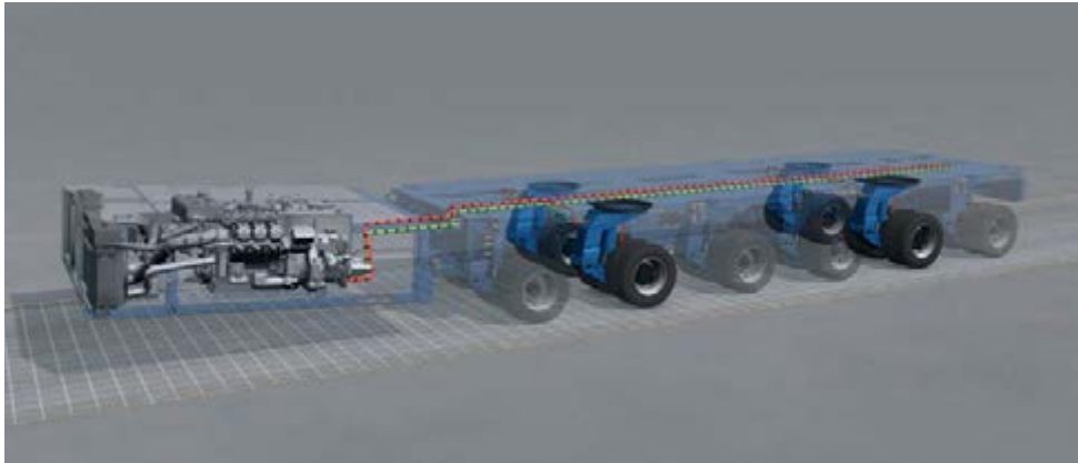
Hydrostatic drive
