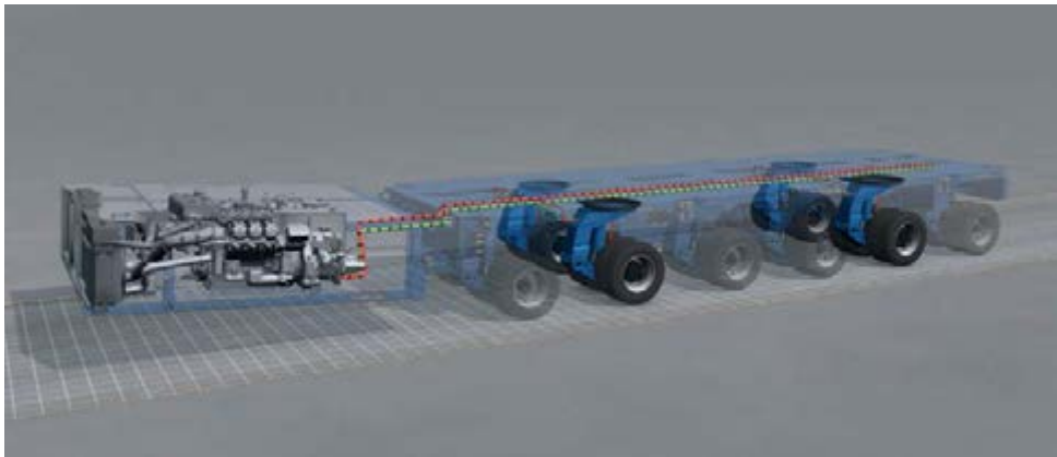
Hydrostatic drive
